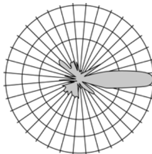
Azimuth radiation pattern
