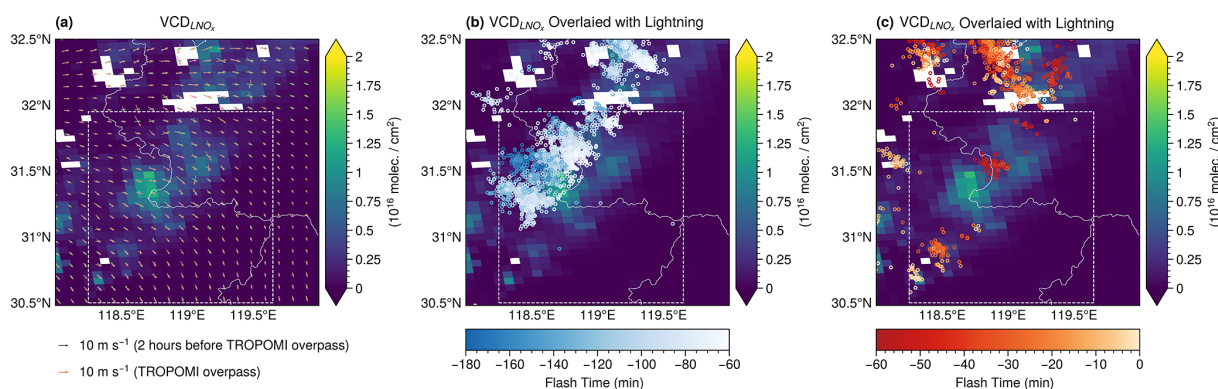
Figure 9. The background is the distribution of LNO x vertical column densities ( \text{VCD}_{\text{LNO}_x} ). The white rectangles are manually selected regions for the LNO x PE estimation. The overlaid wind arrows in (a) are the 500 hPa horizontal wind simulated by WRF-Chem. The lightning dots in (b) and (c) are the flashes whose color depends on the occurrence time relative to the TROPOMI overpass time.
