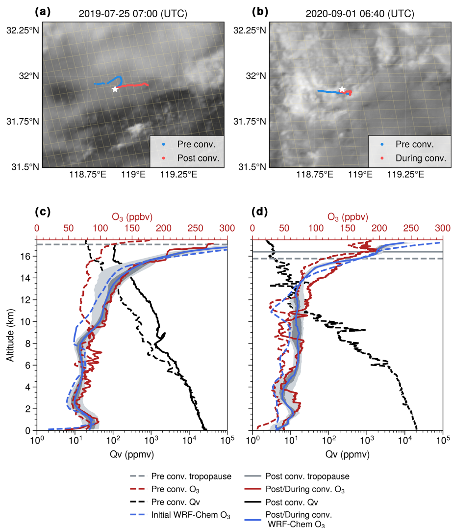
Figure 1. (a, b) The convection detected by the FY-4A Advanced Geostationary Radiation Imager (AGRI) visible channel ( 0.65\ \mu\text{m} ) field at the time when the post-convection/during-convection ozonesondes reached around 10 km. The pre-convection ozonesonde trajectories are colored blue, while the others are in red. The white star symbol stands for the observation station, and the thin yellow lines are the TROPOMI swath pixels. Panels (c) and (d) are the observed O 3 (red) and Qv (black) profiles in the pre-convection (dashed) and post-convection/during-convection (solid) periods. The initial (dashed) and simulated post-convection or during-convection (solid) O 3 profiles are in blue. The dark gray shading is the 50 % confidence interval, while the light one is the 90 % confidence interval. The gray lines are the lapse rate tropopauses.
