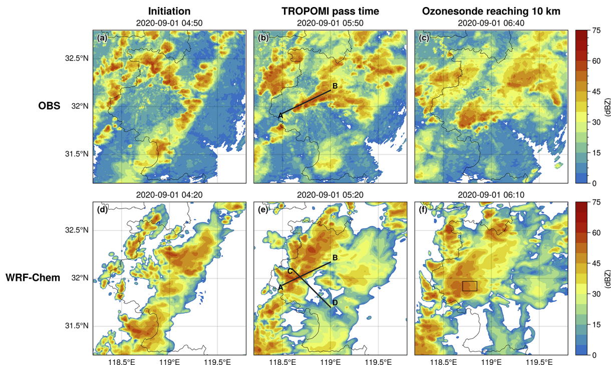
Figure 3. Same as Fig. 2 but for the case on 1 September 2020. The simulation time is 30 min ahead of each radar observation.
