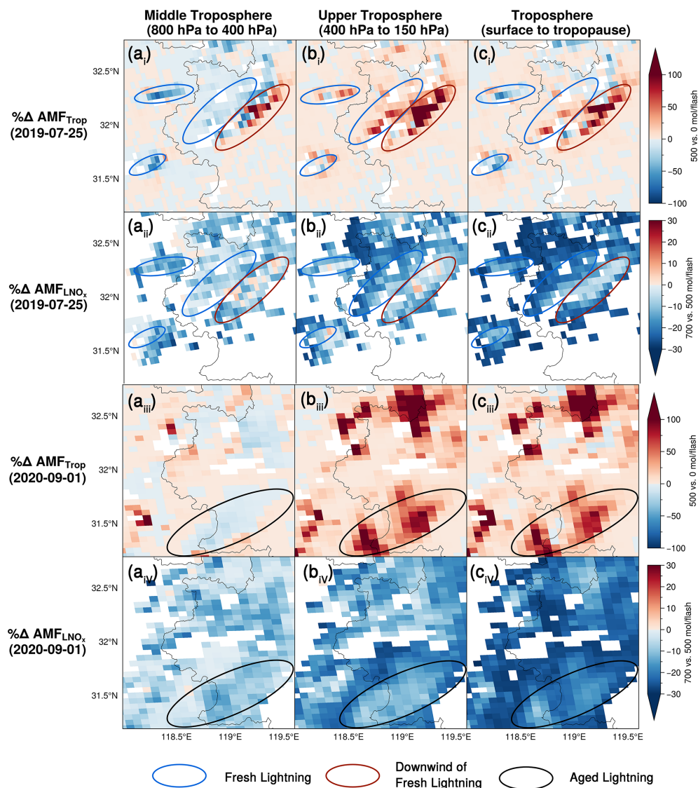
Figure 7. The percent differences of AMFs by replacing the a priori NO 2 profiles at three layers: middle troposphere (left), upper troposphere (middle), and troposphere (right). \Delta\text{AMF}_{\text{Trop}} is the comparison of the \text{AMF}_{\text{Trop}} with 500 mol NO per flash relative to 0 mol NO per flash. \Delta\text{AMF}_{\text{LNO}_x} is the comparison of the \text{AMF}_{\text{LNO}_x} with 700 mol NO per flash relative to 500 mol NO per flash. Three regions are annotated: fresh lightning (blue), downwind of fresh lightning (red), and aged lightning (black). Because of the quite large \text{AMF}_{\text{LNO}_x} values in pixels with little lightning, \Delta\text{AMF}_{\text{LNO}_x} is shown over pixels where 0 < \text{AMF}_{\text{LNO}_x} < 10 .
