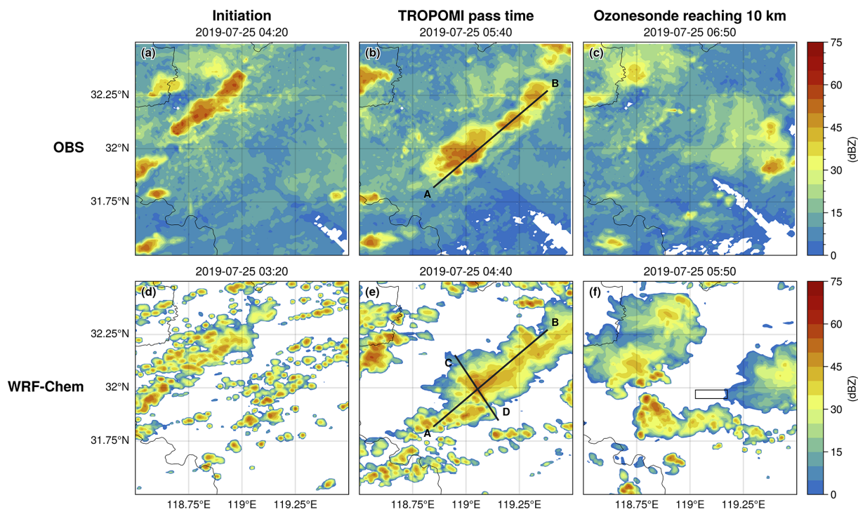
Figure 2. Observed radar composite reflectivity at (a) 04:20, (b) 05:40, and (c) 06:50 UTC. (d–e) WRF-Chem simulated composite reflectivity 1 h before the radar observation times. The A–B solid lines in (b) and (e) are cross-section lines for Fig. S3. The C–D solid line in (e) is the cross-section line for Fig. 4b. The black rectangle is the region for the comparison with ozonesonde.
