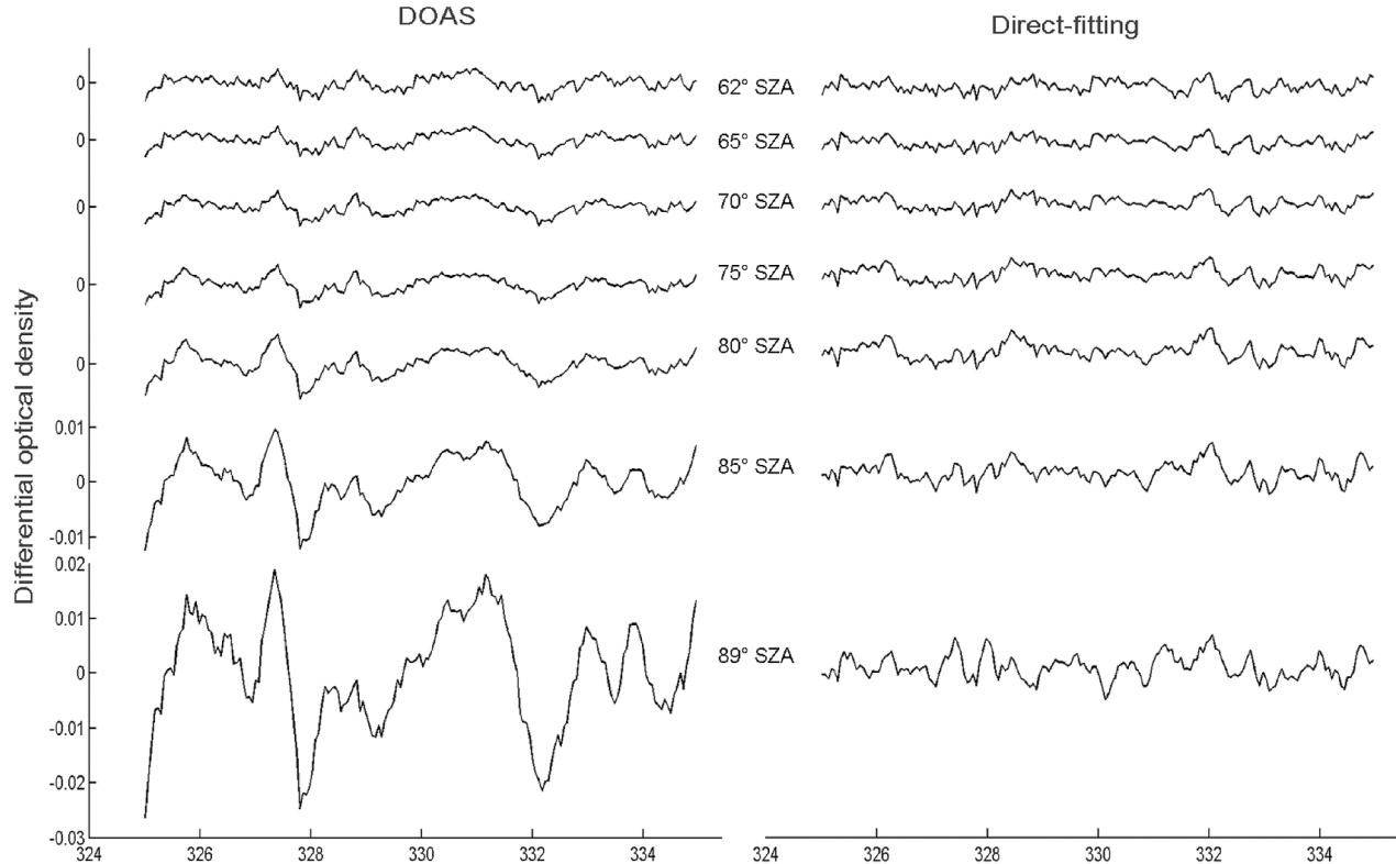
Figure 6. Comparison of total ozone fitting residuals obtained using the DOAS and direct-fitting retrieval schemes, for increasing values of the solar zenith angle. Poorly fitted ozone results typical of DOAS retrievals at low sun are strongly reduced with the direct-fitting approach.
