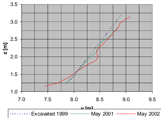
Fig. 18. Reduction in slope angle due to weathering, erosion and ravelling of the slope of Fig. 17
