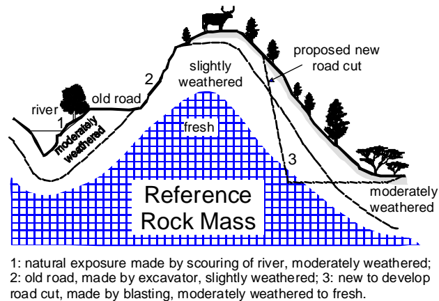
Fig. 4. Sketch of exposures in rock masses with various degrees of weathering, different types of excavation, and showing the concept of the 'reference rock mass'.
