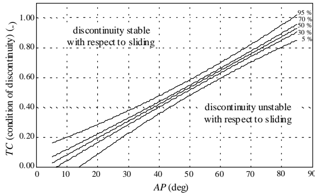
Fig. 5. Sliding criterion.
