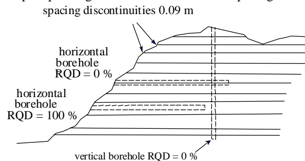
Fig. 2. Bias of RQD due to orientation of borehole.
