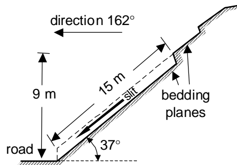
Fig. 10. Plane sliding in a limestone slope of example II
