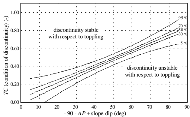
Fig. 6. Toppling criterion
