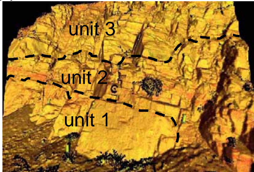
Fig. 16. Rendered image of an exposure scanned with Lidar (modified after Slob et al, 2002, acknowledged are Roger Moore of 3D Scan - A Cyrax Service Provider, and Jerry Higgins, Colorado School of Mines, USA, for providing the image)
