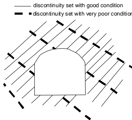
Fig. 3. Influence of discontinuity condition. It is not clear which discontinuity set has the worst influence on the stability of the tunnel.
