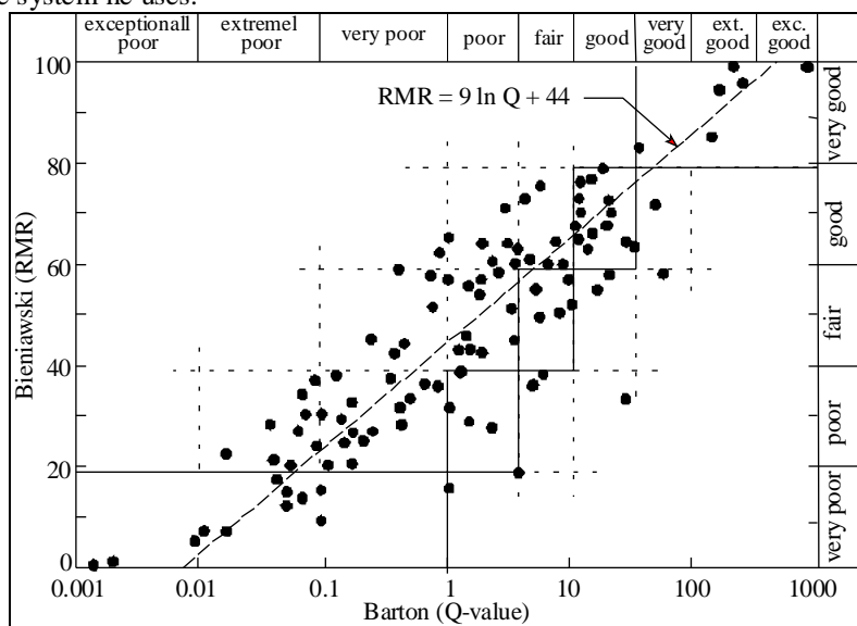
Fig. 1. Correlation between Bieniawski (RMR) and Barton (Q). Data from case histories with RMR and Q-system (after Bieniawski, 1989). (Continuous lines indicate correlating classes of rock mass quality.)
