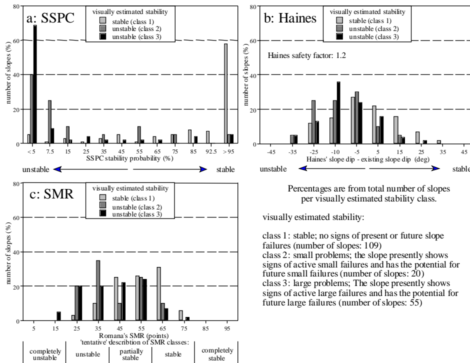
Fig. 8. Comparison of slope stability assessment by different classification systems.
