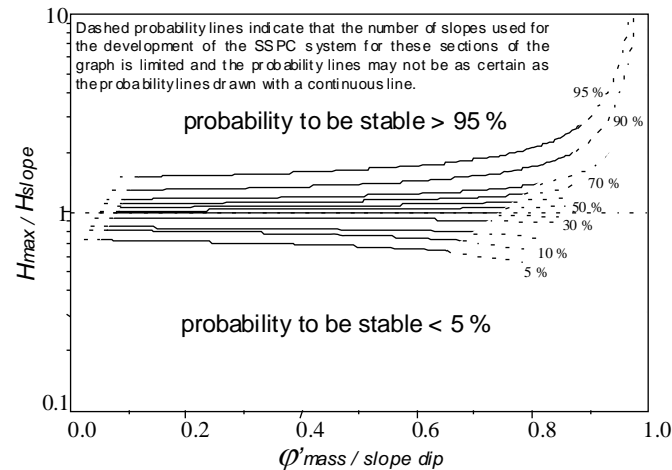
Fig. 7. Probability of orientation independent stability.
