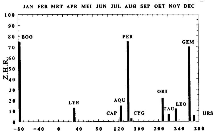
Figure 1: ZHR meteoroorzwermen in 1990
