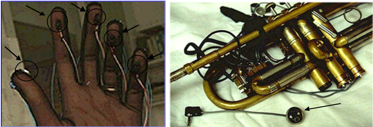
Fig. 24. Lady's Glove sensors (left) and Jonathan Impett's metatrumpet's sensors (right).
