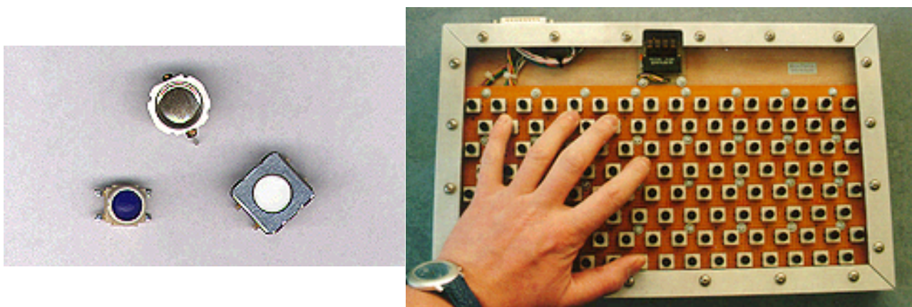
Fig. 13. Switches (left) and Clavette microtonal keyboard (right).
