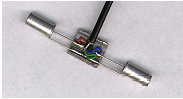
Fig. 29. A pair of tilt switches.
