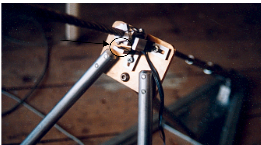
Fig. 25. The 'bridge' of the Global String instrument.
