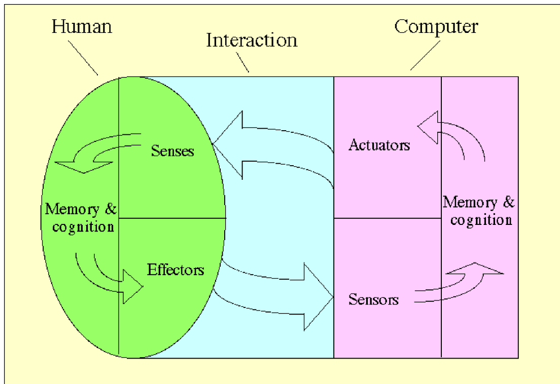
Fig. 1. Human-Machine Interaction.
