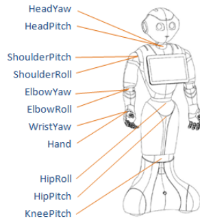
Figure 1: Pepper robot joints, 17 DOF
